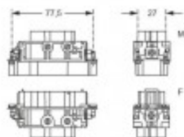
contacts side (front view)
